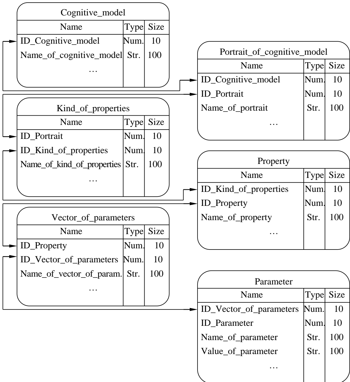
Picture 4.7. The infological scheme of database
